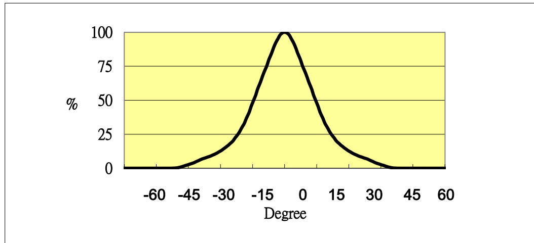
Relative Intensity of QR06230-C1C-BESQ
