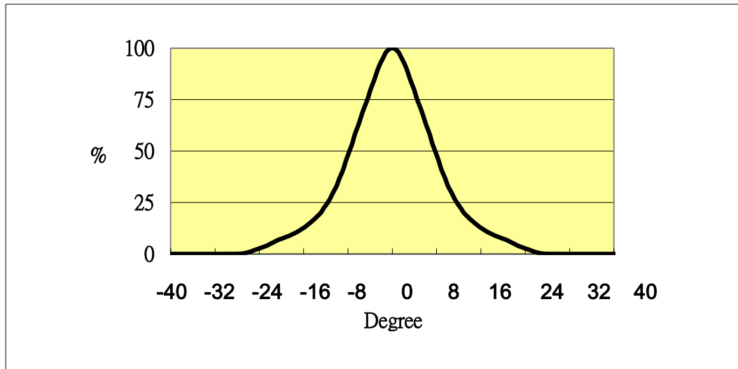
Relative Intensity of QR06215-C1C-BESQ
