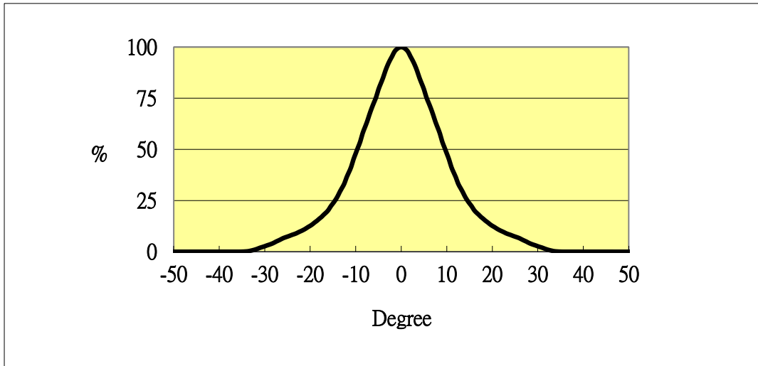
Relative Intensity of QR05025-C1C-BESQ
