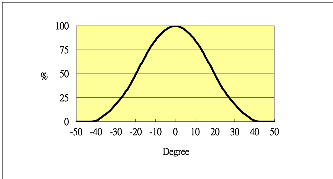
Relative Intensity of QR05040-C1C-BESQ
